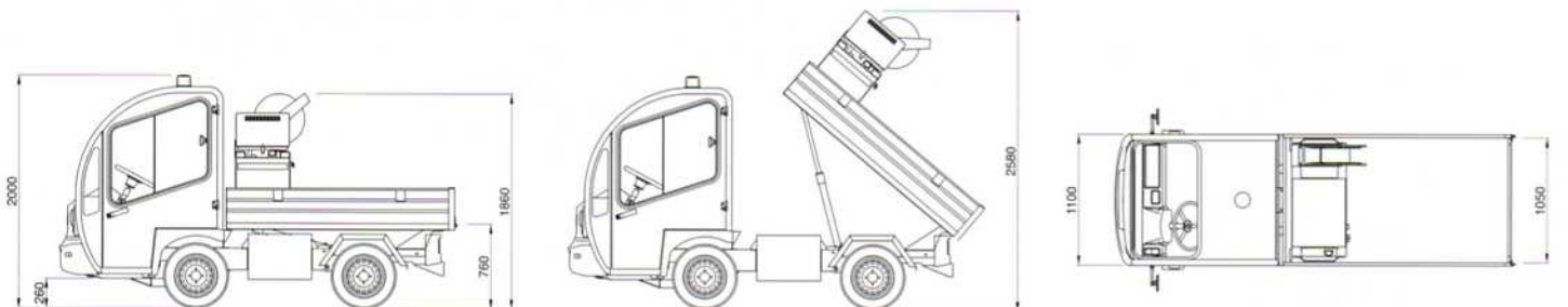
Compact version 200 l
