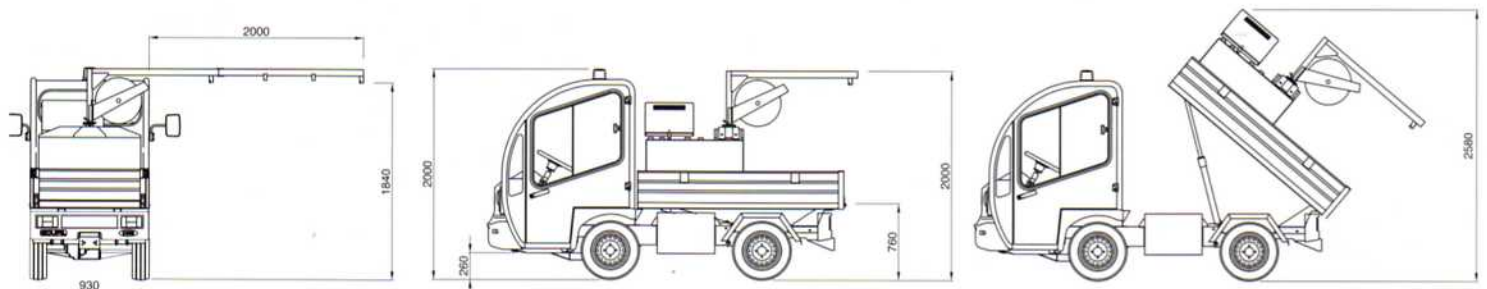
400 l version with extension arm
